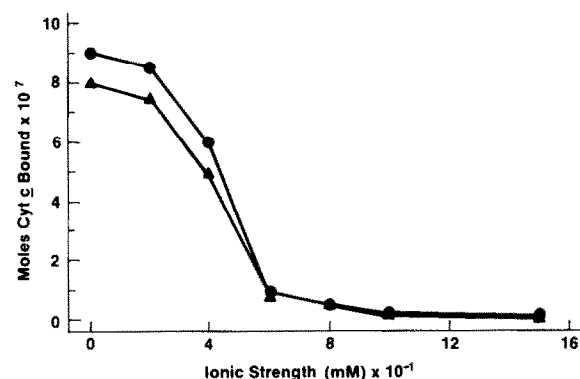
Fig.1. Binding of equine and yeast cytochromes c to a C. vinosum flavocytochrome c -552-Affigel 10 affinity column. Either 900 nmol equine cytochrome c (●) or 800 nmol yeast ( S. cerevisiae ) cytochrome c (▲) in 20 mM Tris buffer (pH 8.0) was applied to the affinity column (bed volume 3.0 ml) which had been pre-equilibrated with the same buffer. The ionic strength of the eluting buffer was increased by NaCl addition. 2.0-ml fractions were collected. Total recovery of each cytochrome was approx. 95%.
